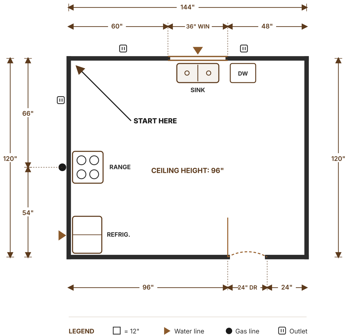
Sample kitchen layout — yours may differ. Note walls, windows, doors (and the way they swing), plus water, gas & electrical lines.
